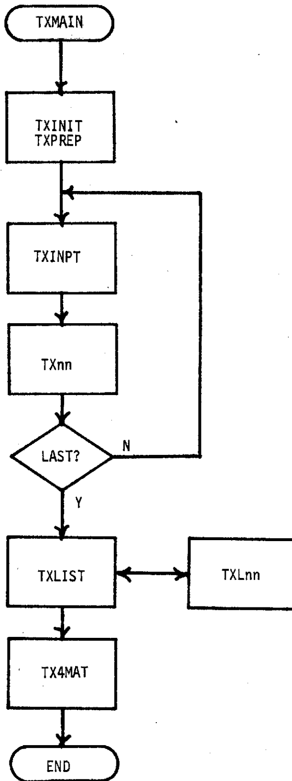
INTERPRETIVE TRANSLATOR PROGRAM STRUCTURE
